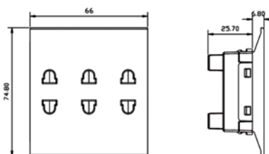
EURO-AMERICAN 3 SOCKETS WITH SHUTTER (66mm) Code: NUV 80 233
