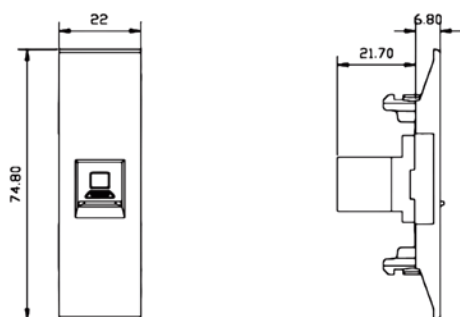
COMPUTER SOCKET CAT6 WITH SHUTTER (22mm) Code: Nov 80 684
