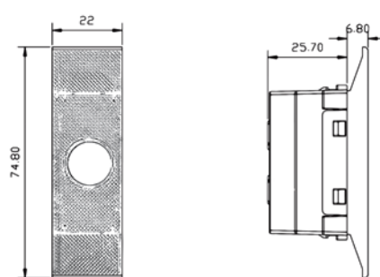
EMERGENCY LIGHT (22mm) Code: NUV 80 833
