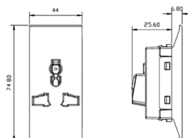
UNIVERSAL SOCKET WITH SHUTTER (44mm) Code: NUV 80 220
