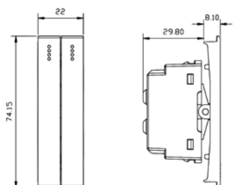
THIN SWITCH ONE WAY - 22mm Code: NUV 80 581
