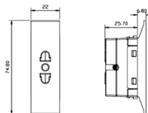
EURO-AMERICAN SOCKET WITH SHUTTER AND EARTH (22mm) Code: NUV 80 214
