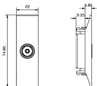
SATELLITE SOCKET (22mm) Code: NUV 80 252
