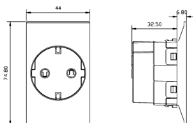
GERMAN SOCKET WITH SHUTTER (44 mm) Code: NUV 80 265
