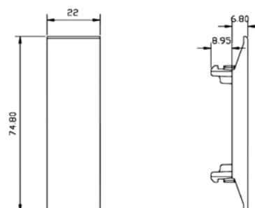
BLANK 22mm Code: NUV 80 056
