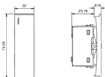
ONE WAY SWITCH - 22mm Code: NUV 80 571
