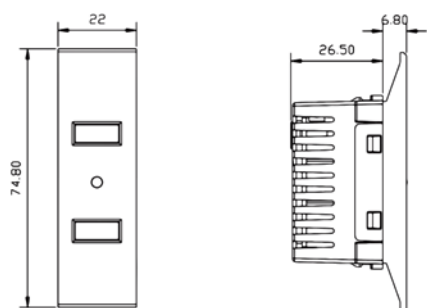
TWO USB SOCKET CHARGER (22mm) Code: NUV 80 907
