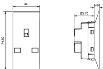
BRITISH SOCKET WITH SHUTTER (44mm) Code: NUV 80 208
