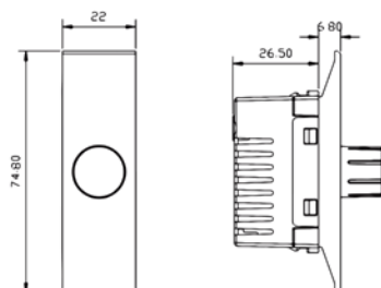
LIGHT DIMMER LED (22mm) Code: Nov 80 803
