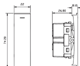
ONE WAY SWITCH WITH LAMP 22mm Code: NUV 80 572
