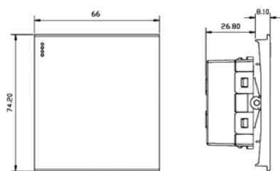
ONE GANG ONE WAY SWITCH (66mm) Code: NUV 80 573
